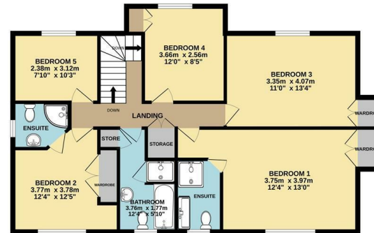
1ST FLOOR 90.7 sq.m. (977 sq.ft.) approx.
